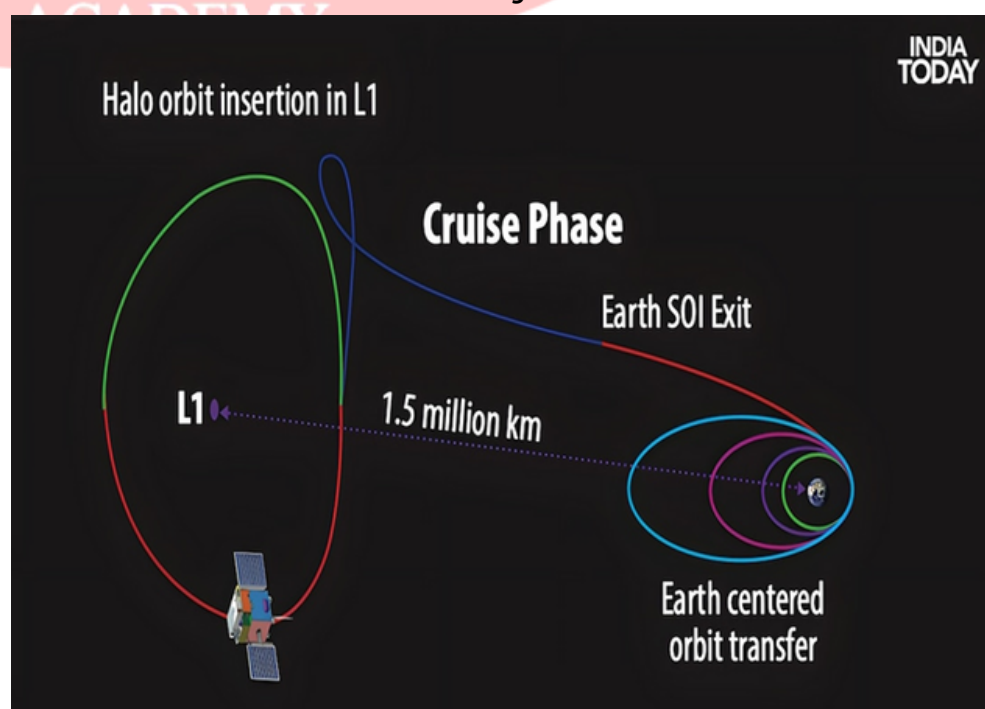
Orbit of Aditya L1
