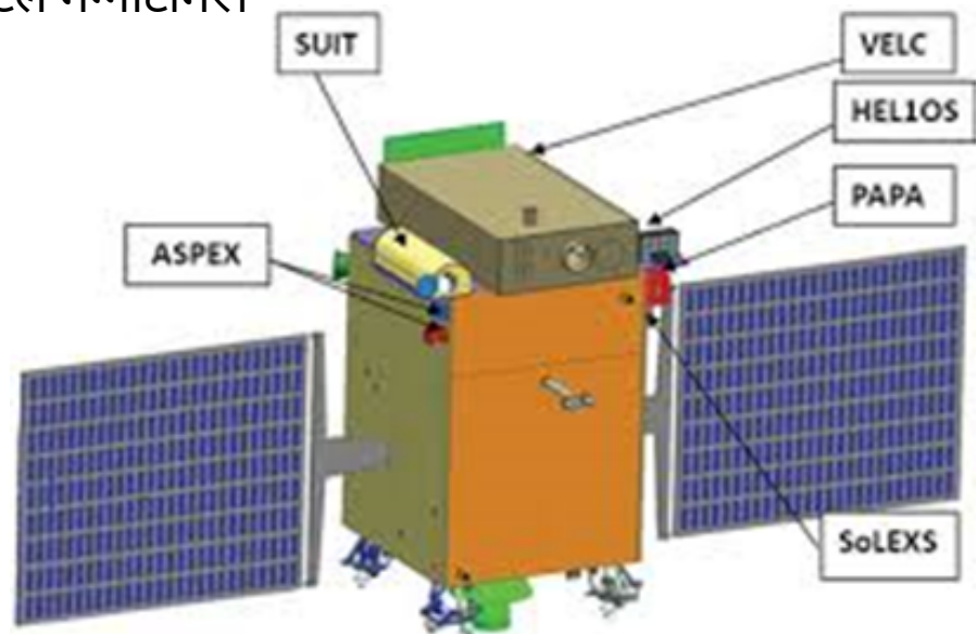
Schematic layout of proposed Aditya-L1 Spacecraft
